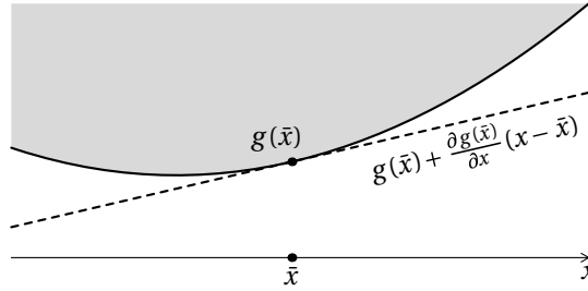
FIGURE A.4: A C^1 function g : \mathbb{R} \rightarrow \mathbb{R} is convex iff g(x) \geq g(\bar{x}) + \frac{\partial g(\bar{x})}{\partial x}(x - \bar{x}) \forall \bar{x}, x \in \mathbb{R} . See Lemma A.7.1.
