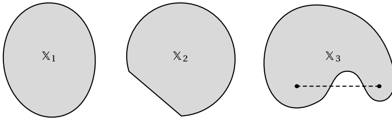
FIGURE A.2: Three subsets of \mathbb{R}^2 . Sets X_1, X_2 are convex. The third set, X_3 , is not convex because one of its line segments is not contained in X_3 . See § A.7.
