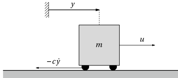
FIGURE 4.6: A car at position y subject to a friction force -c\dot{y} and external force u . See Example 4.6.4.
