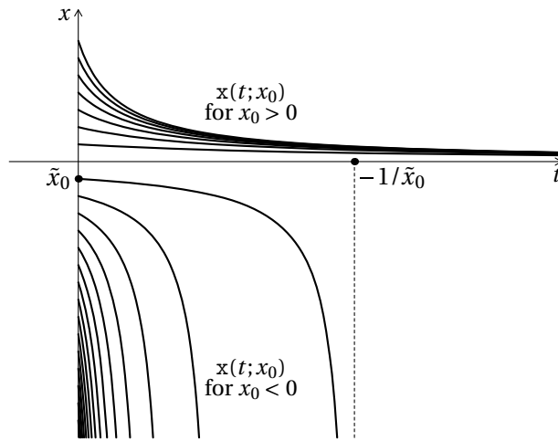
FIGURE B.2: Solutions x(t; x_0) of \dot{x}(t) = -x^2(t) for various initial states x(0) = x_0 . If x_0 < 0 then the solution escapes at t = -1/x_0 . See Example B.1.5.
