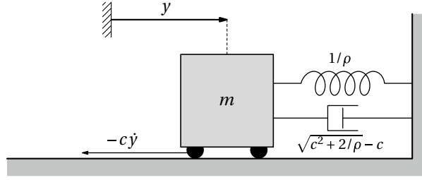
FIGURE 4.7: A car at position y subject to a friction force -c\dot{y} . It is optimally controlled with a spring with spring constant 1/\rho and a damper with friction coefficient \sqrt{c^2 + 2/\rho} - c . See Example 4.6.4.
