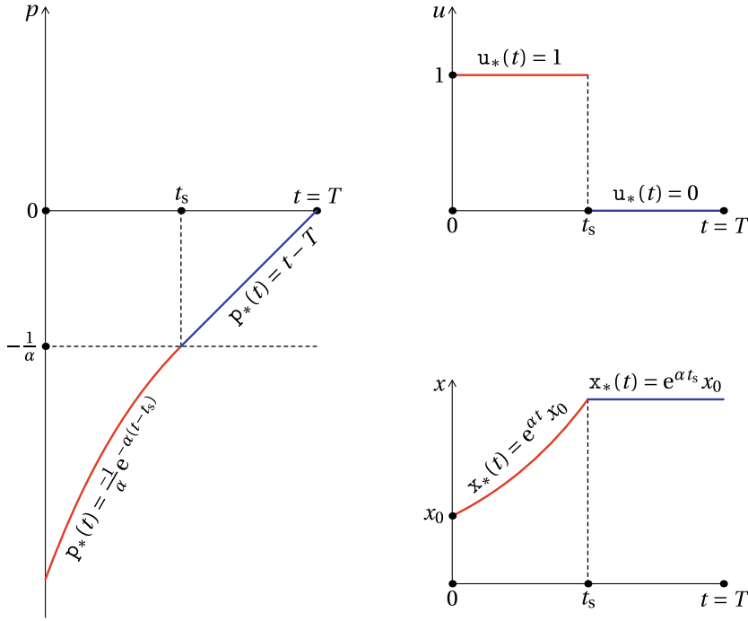
FIGURE 2.2: Optimal costate p_*(t) , optimal input u_*(t) and optimal state x_*(t) . See Example 2.5.5.
