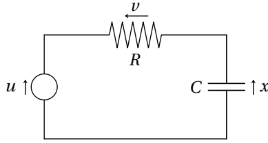
FIGURE 2.9: An RC -circuit with resistance R and capacitance C . The voltage source is denoted by u , and the voltage across the capacitor is denoted by x . See Exercise 2.9.
