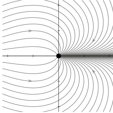
FIGURE B.8: Phase portrait of the system of Example B.3.6. The origin is globally asymptotically stable.
