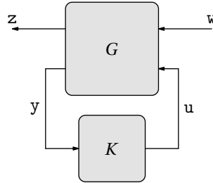
FIGURE 5.2: Configuration for the standard \mathbb{H}_\infty problem.
