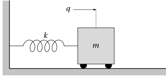
FIGURE 1.13: A mass m attached to a linear spring with spring constant k . See Example 1.3.3.
