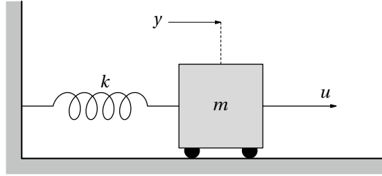
FIGURE 4.4: Car connected to a wall via a spring and with a force control u . See Example 4.6.3.
