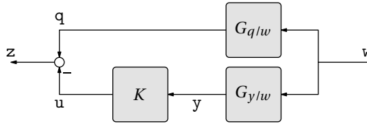
FIGURE 5.1: Filtering configuration. See Example 5.1.3.
