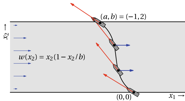
FIGURE 2.6: The problem of Zermelo. We assume that the speed of the boat with respect to the water is v = 1 and that the flow velocity is w(x_2) = x_2(1 - x_2/b) with (a, b) = (-1, 2) . The optimal trajectory x_{*1}(t), x_{*2}(t) as shown here was computed by iterating over u_0 in (2.36). The optimal value is u_0 = 2.5937 , and the optimal (minimal) time is T = 2.7570 . The optimal angle u_*(t) of the boat does not vary much with time. See Example 2.7.2.
