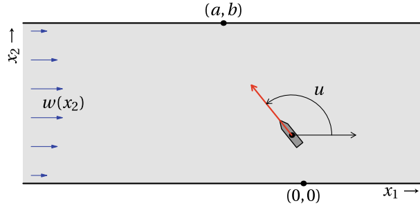
FIGURE 2.4: The problem of Zermelo. See Example 2.7.2.
