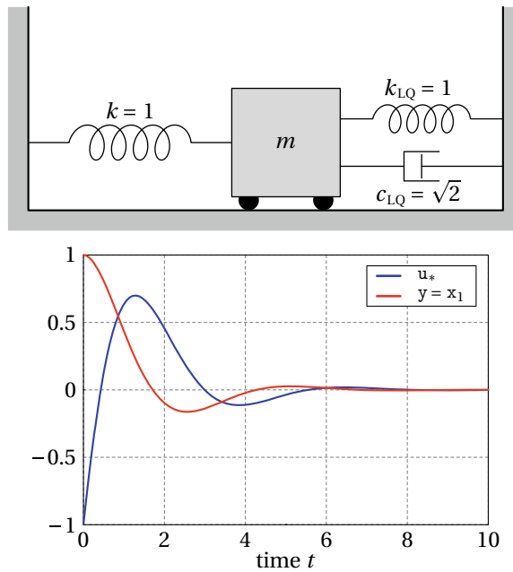
FIGURE 4.5: Top: a car connected to a wall via a spring (on the left). The car is controlled with an LQ-optimal force u_*(t) = -k_{LQ}y(t) - c_{LQ}\dot{y}(t) implemented as spring/damper system (on the right). Bottom: responses u_*(t) and y(t) = x_1(t) for initial state x(0) = \begin{bmatrix} 1 \\ 0 \end{bmatrix} . See Example 4.6.3.
