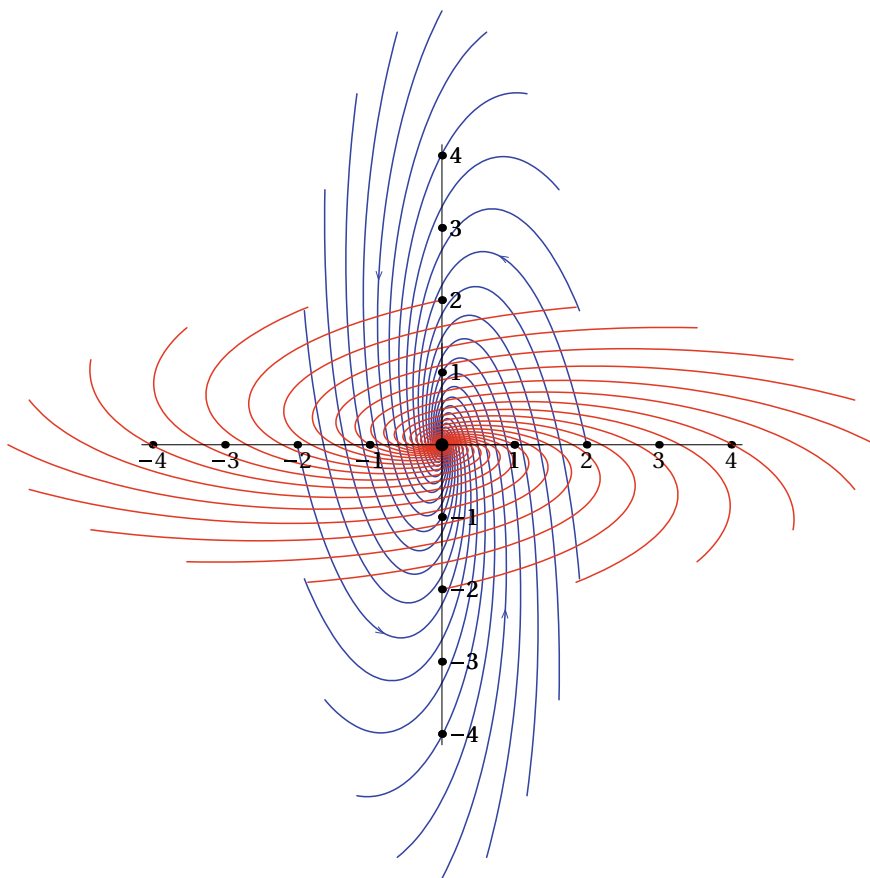
FIGURE B.14: The blue phase portrait is that of the system of Exercise B.22. This is also the phase portrait of the system \dot{\mathbf{x}}(t) = A_{\text{even}}\mathbf{x}(t) of Exercise B.23. In red is the phase portrait of \dot{\mathbf{x}}(t) = A_{\text{odd}}\mathbf{x}(t) of Exercise B.23. All trajectories (blue and red) converge to zero as t \rightarrow \infty .
