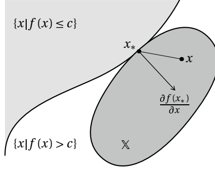
FIGURE A.5: Let f : \mathbb{R}^2 \rightarrow \mathbb{R} , and \mathbb{X} \subseteq \mathbb{R}^2 . If \mathbb{X} is convex, and x_* minimizes f(x) over all x \in \mathbb{X} , then \frac{\partial f(x_*)}{\partial x^T}(x - x_*) \geq 0 \forall x \in \mathbb{X} . See Lemma A.7.3.
