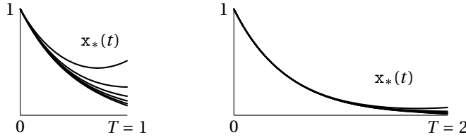
FIGURE 4.11: Graphs of optimal x_* with x_0 = 1 . Left: for T = 1 and s = 0, 1, 2, 3, 4, 5 . Right: for T = 2 and s = 0, 1, 2, 3, 4, 5 . See Exercise 4.7.
