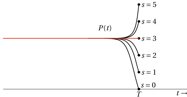
FIGURE 4.10: Graph of P(t) for several values of P(T) = s . If s = 3 then P(t) is constant (shown in red). See Exercise 4.7.
