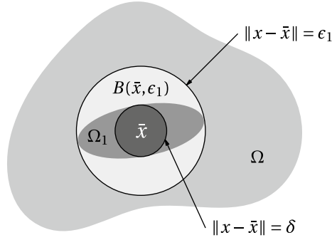
FIGURE B.5: Four inclusions of regions (used in the proof of Theorem B.3.2).
