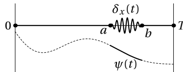
FIGURE 1.15: About the construction of a \delta_x(t) that violates (1.51). See the proof of Lemma 1.6.2.
