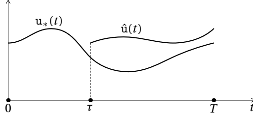
FIGURE 3.1: Principle of optimality, see § 3.2.
