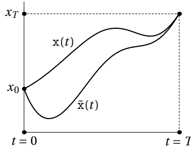
FIGURE 1.5: Two functions x, \tilde{x} : [0, T] \rightarrow \mathbb{R} that satisfy the boundary conditions (1.12).
