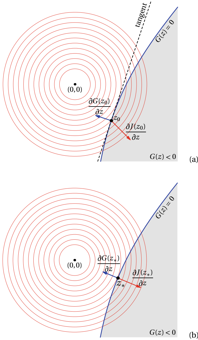
FIGURE A.6: Let J(z) = z_1^2 + z_2^2 . Its level sets \{z = (z_1, z_2) | J(z) = c\} are circles (shown in red). Suppose the blue curve is where G(z) = 0 and the gray region is where G(z) < 0 . The z_0 in (a) is not a local minimizer of J(z) subject to G(z) = 0 . The z_* in (b) is a local minimizer, and it satisfies the first-order condition that the gradients \partial J(z)/\partial z and \partial G(z)/\partial z are aligned at z = z_* . See § A.8.
