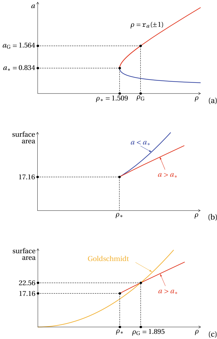
FIGURE 1.11: (a) The endpoint radius r_a(\pm 1) := a \cosh(1/a) of the catenoid as a function of a . Its minimal value r_a(\pm 1) is \rho_* = 1.509 (attained at a_* = 0.834 ); (b) the area of the catenoid as a function of endpoint radius \rho ; (c) the area of the catenoid (in red) and of the Goldschmidt solution (in yellow) as a function of endpoint radius \rho . The two areas are the same at \rho_G = 1.895 . This \rho_G corresponds to a_G = 1.564 (see part (a) of this figure). See Example 1.3.2.
