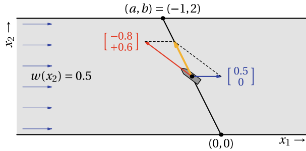
FIGURE 2.5: The problem of Zermelo. We assume that the speed of the boat with respect to the water is v = 1 and that the flow velocity is w(x_2) = 0.5 , and (a, b) = (-1, 2) . Then optimal is to take u constant such that \begin{bmatrix} \cos(u) \\ \sin(u) \end{bmatrix} = \begin{bmatrix} -0.8 \\ +0.6 \end{bmatrix} (shown in red), for then the sum of \begin{bmatrix} \cos(u) \\ \sin(u) \end{bmatrix} and \begin{bmatrix} 0.5 \\ 0 \end{bmatrix} (shown in blue) is \begin{bmatrix} -0.3 \\ 0.6 \end{bmatrix} (shown in yellow), and this direction brings the boat to (a, b) = (-1, 2) as required. It takes T = b/0.6 = 3\frac{1}{3} units of time. See Example 2.7.2.
