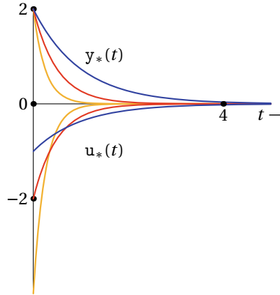
FIGURE 4.2: Graphs of optimal y_* and u_* for \rho = 1/2 (yellow), for \rho = 1 (red), and \rho = 2 (blue). The larger \rho is the slower the system is and the smaller |u_*(0)| is. See Example 4.6.1.
