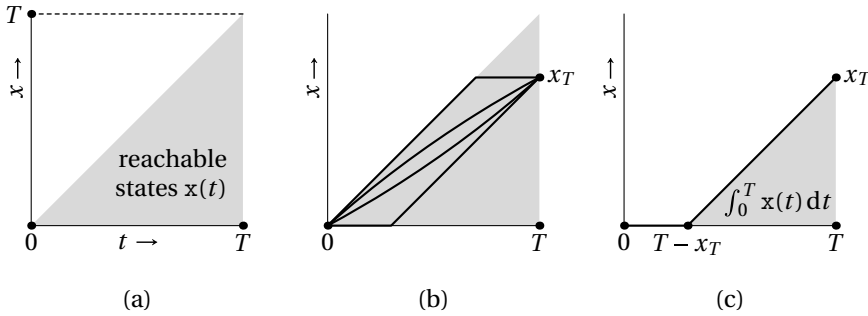
FIGURE 2.1: Reachable states and candidate optimal states for the optimal control problem of Example 2.1.1.
