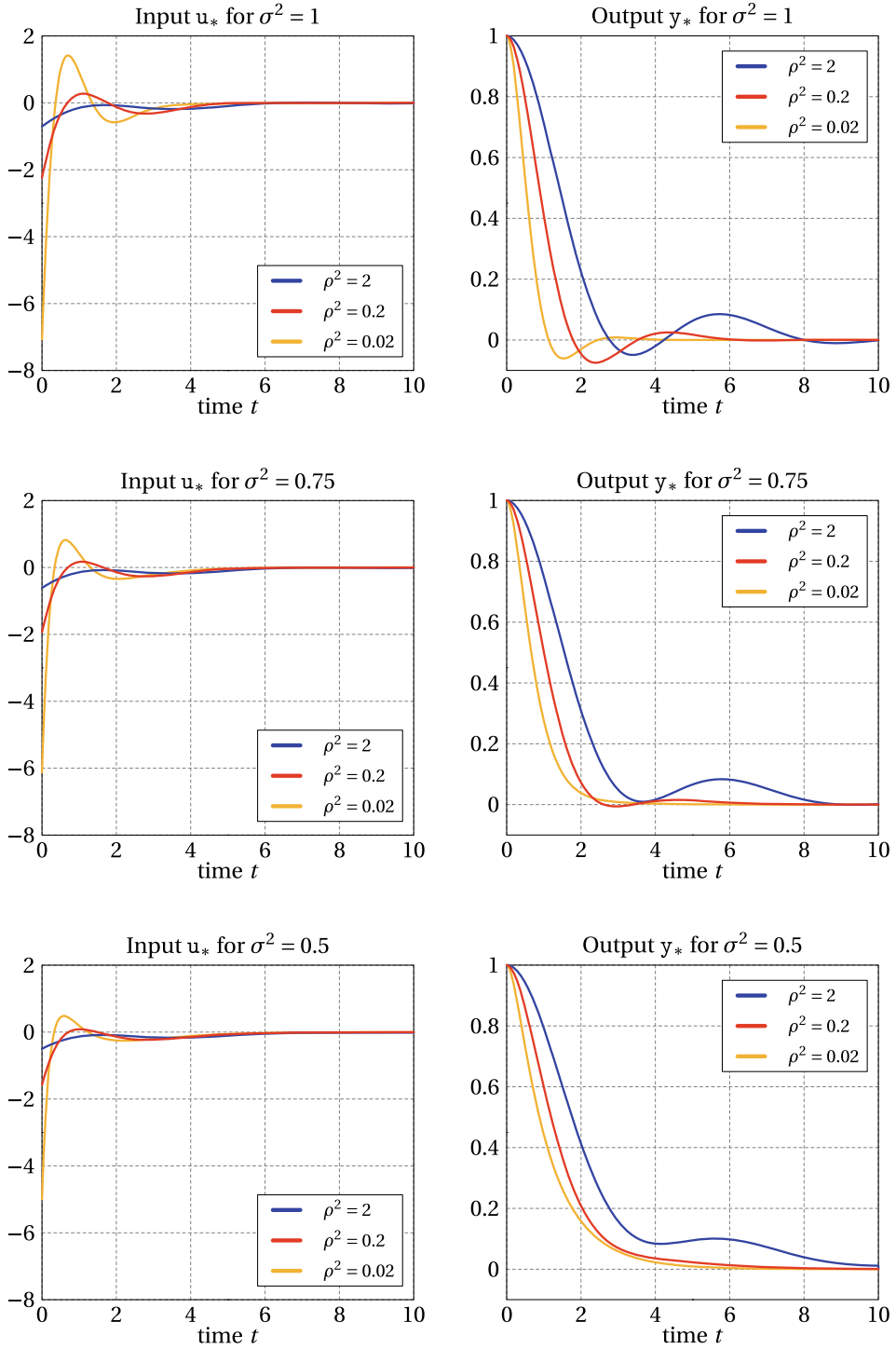
FIGURE 4.3: LQ-optimal responses of u_* (left) and y_* (right) for various combinations of \sigma \in [0, 1] and \rho > 0 . See Example 4.6.2.
