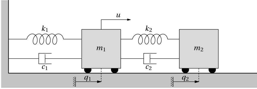
FIGURE 4.8: Two connected cars. The purpose is to control the second car with a force u that acts on the first car. See Example 4.6.5.
