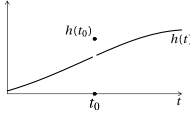
FIGURE 2.3: Suppose a function h : \mathbb{R} \rightarrow \mathbb{R} is not continuous at some t_0 , but that the limit from the left and from the right at t_0 are the same: \lim_{t \uparrow t_0} h(t) = \lim_{s \downarrow t_0} h(s) . Then the discontinuity of h at t_0 is said to be removable . See the proof of Theorem 2.5.6.
