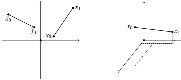
FIGURE A.1: Left: two line segments in \mathbb{R}^2 . Right: one line segment in \mathbb{R}^3 . See § A.7.
