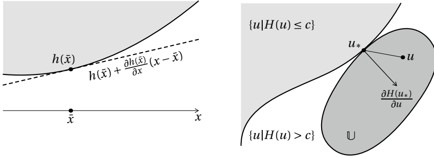
FIGURE 2.7: Left: a C^1 function h: \mathbb{R} \rightarrow \mathbb{R} is convex iff h(x) \geq h(\bar{x}) + \frac{\partial h(\bar{x})}{\partial x}(x - \bar{x}) \forall \bar{x}, x \in \mathbb{R} . Right: Suppose H: \mathbb{R}^2 \rightarrow \mathbb{R} is C^1 and that \mathbb{U} \subseteq \mathbb{R}^2 . If H(u_*) = \min_{u \in \mathbb{U}} H(u) for some u_* \in \mathbb{U} , and \mathbb{U} is convex, then \frac{\partial H(u_*)}{\partial u^T}(u - u_*) \geq 0 \forall u \in \mathbb{U} . This is used in the proof of Theorem 2.8.1. Appendix A.7 has more details.
