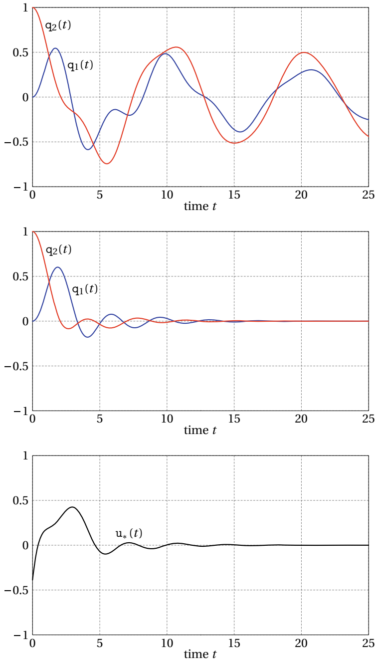
FIGURE 4.9: Top: positions of the uncontrolled cars. Middle: positions of the controlled cars. Bottom: control force u_* for the controlled car. For all cases the initial state is q_1(0) = 0, q_2(0) = 1, \dot{q}_1(0) = 0, \dot{q}_2(0) = 0 . See Example 4.6.5.
