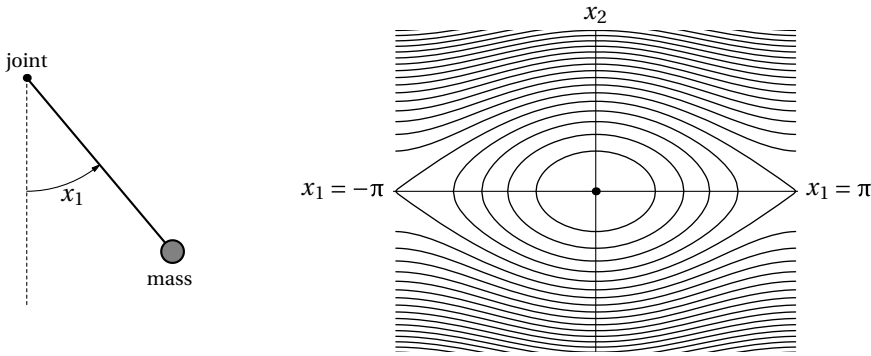
FIGURE B.7: Left: pendulum. Right: level sets of its mechanical energy V(x) . See Example B.3.4.
