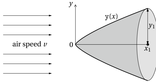
FIGURE 1.17: Solid of least resistance. See Exercise 1.5.
