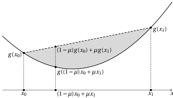
FIGURE A.3: A function g: \mathbb{R} \rightarrow \mathbb{R} is convex (on \mathbb{R} ) if for every x_0, x_1 \in \mathbb{R} and every \mu \in [0, 1] we have g((1-\mu)x_0 + \mu x_1) \leq (1-\mu)g(x_0) + \mu g(x_1) . (In the plot we took \mu = 1/4 .) See § A.7.
