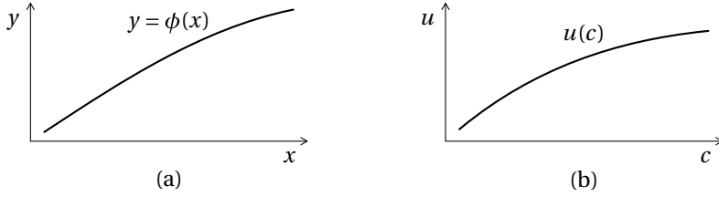
FIGURE 1.4: Left: national product y is concave in capital stock x . Right: utility functions u are strictly concave in consumption c . See Example 1.1.2.
