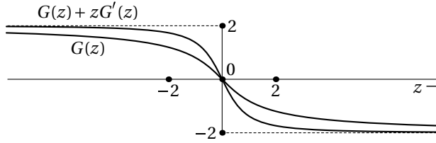
FIGURE 3.4: Graphs of G(z) and G(z) + zG'(z) of the solution of the differential equation G'(z) + 1 - \frac{1}{4} (G(z) + zG'(z))^2 = 0 , G(0) = 0 . See Exercise 3.9.
