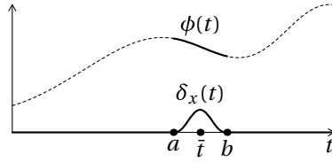
FIGURE 1.7: The function \delta_x(t) defined in (1.21).
